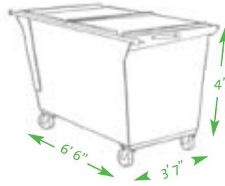
2-Cubic Yard
