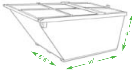
6-Cubic Yard
